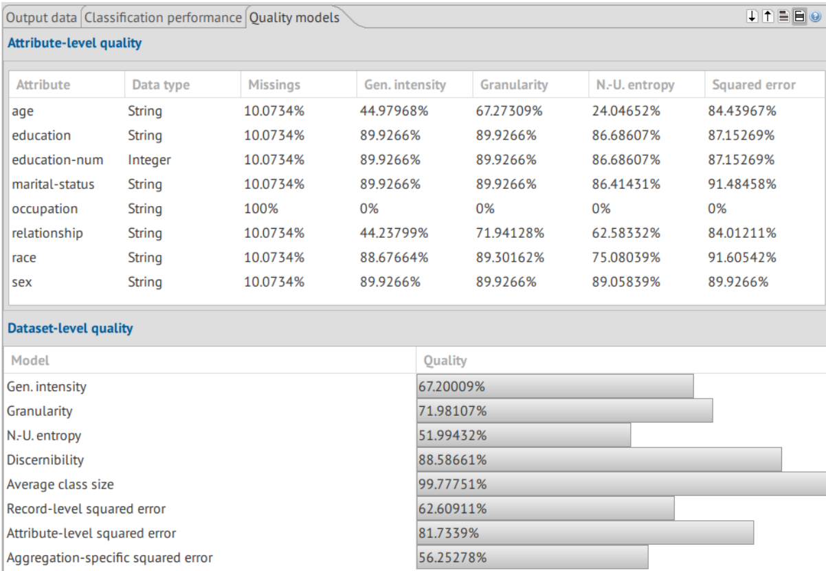
Figure 9: Quality models
